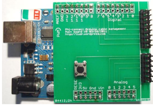
Fig. 3 Connect the main board to Arduino or compatible board.
