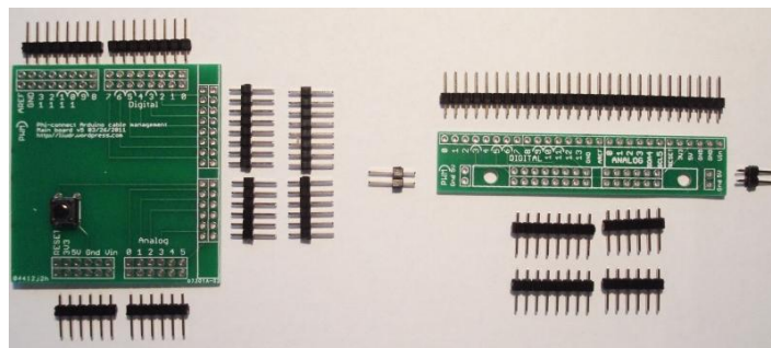
Fig. 2 Phi-connect kit parts (second breakout board and ribbon cable not pictured)
