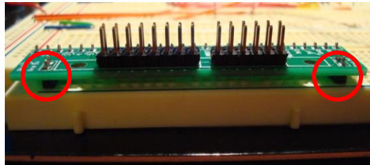
Fig. 5 Make sure that you have inserted the two 2-pin (red circles) firmly into the busses on the side of your board. This powers these busses and stabilizes the breakout board.
