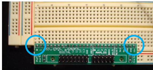
Fig. 4 Insert breakout board on a breadboard per picture, with pin 0 in the first row's left hole (a) and pin Vin in row 28's left hole (a). See the blue circles.
