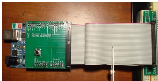
Fig. 6 Connect the main board to the breakout board. Watch the mechanical key when you insert the connectors. THE CABLE STAYS FLAT. DO NOT TWIST IT 180°.
